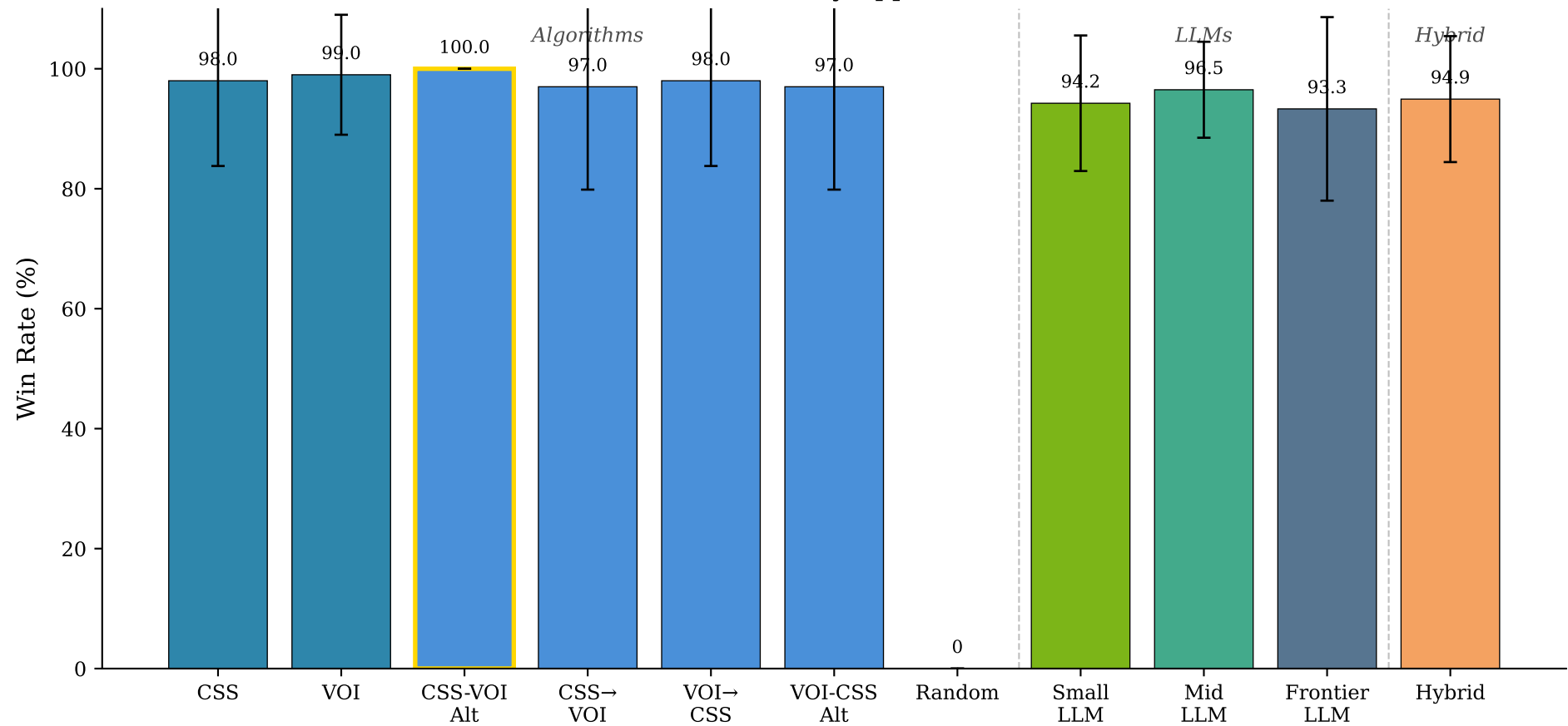
Win Rate by Approach
