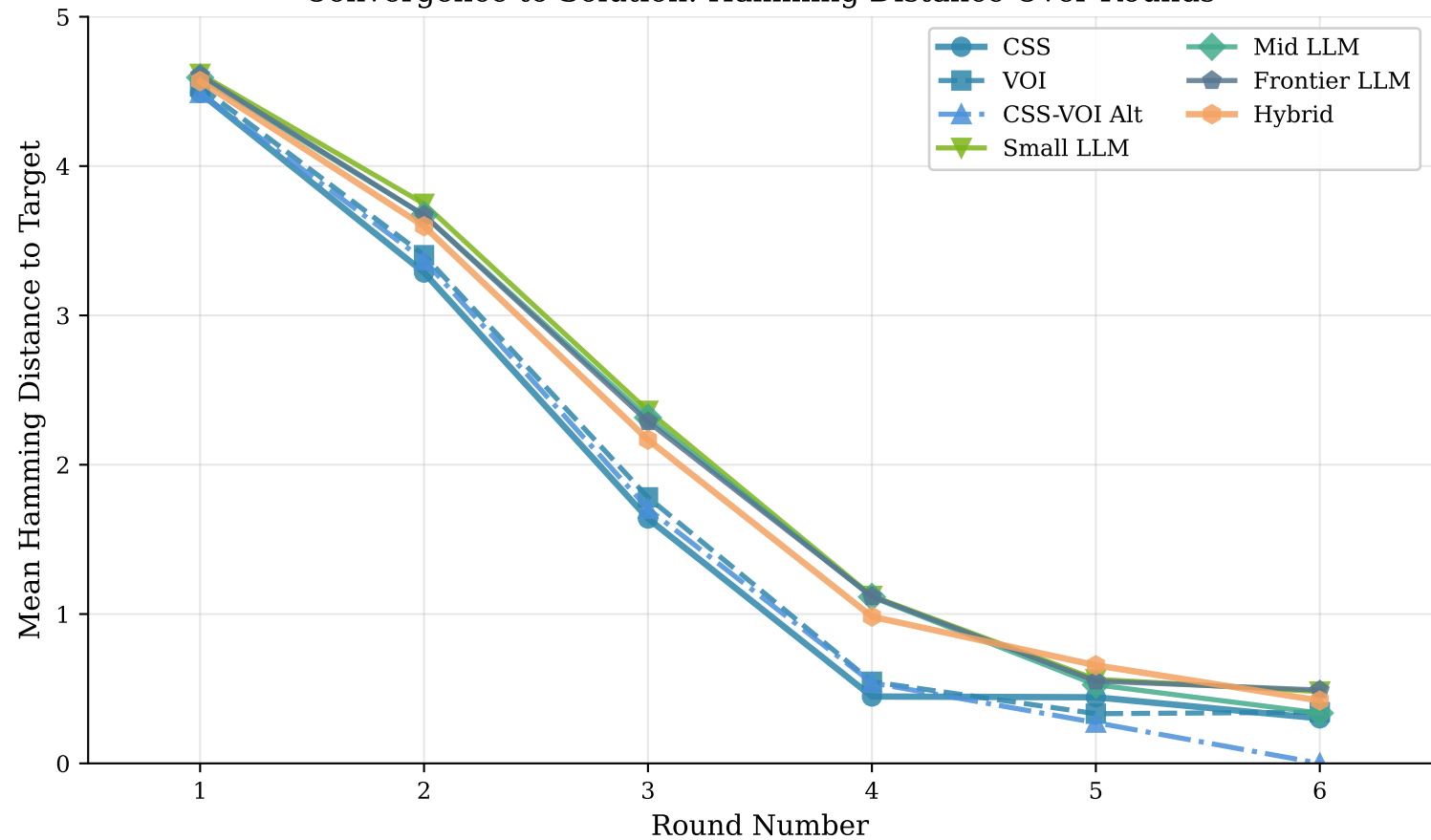
Convergence to Solution: Hamming Distance Over Rounds
