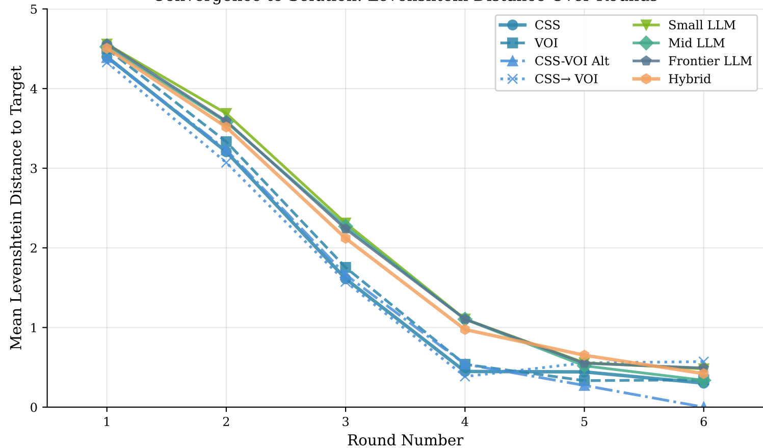
Convergence to Solution: Levenshtein Distance Over Rounds
