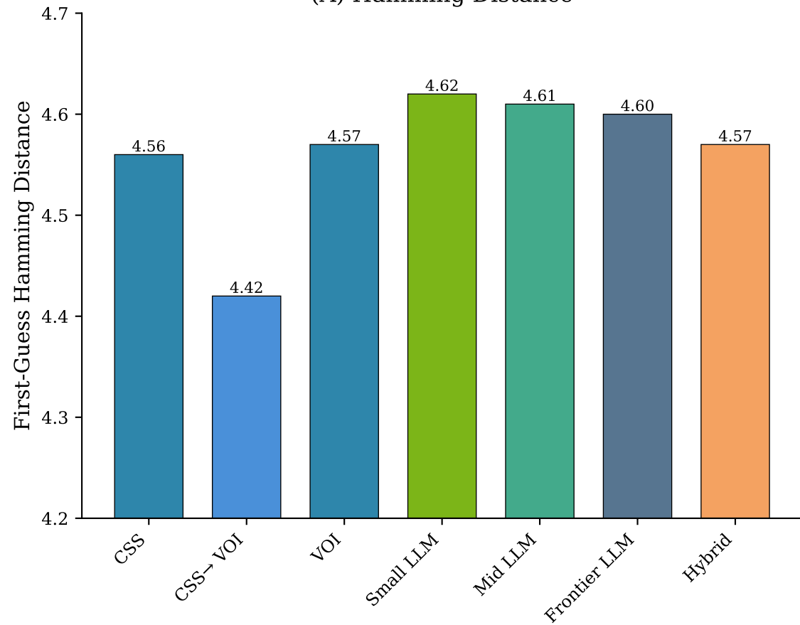
(A) Hamming Distance
