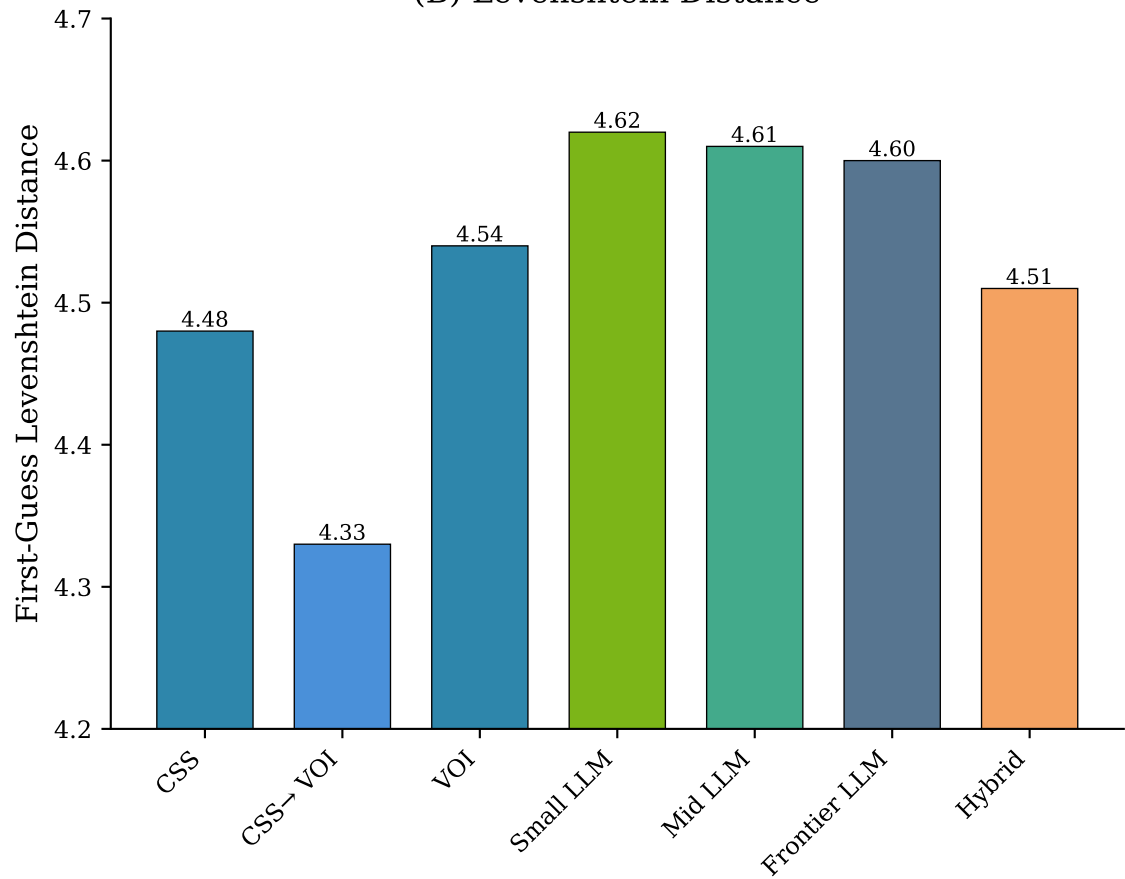
(B) Levenshtein Distance
