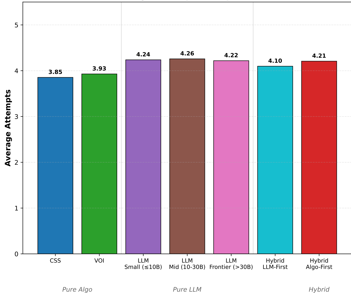
Average Attempts Comparison
