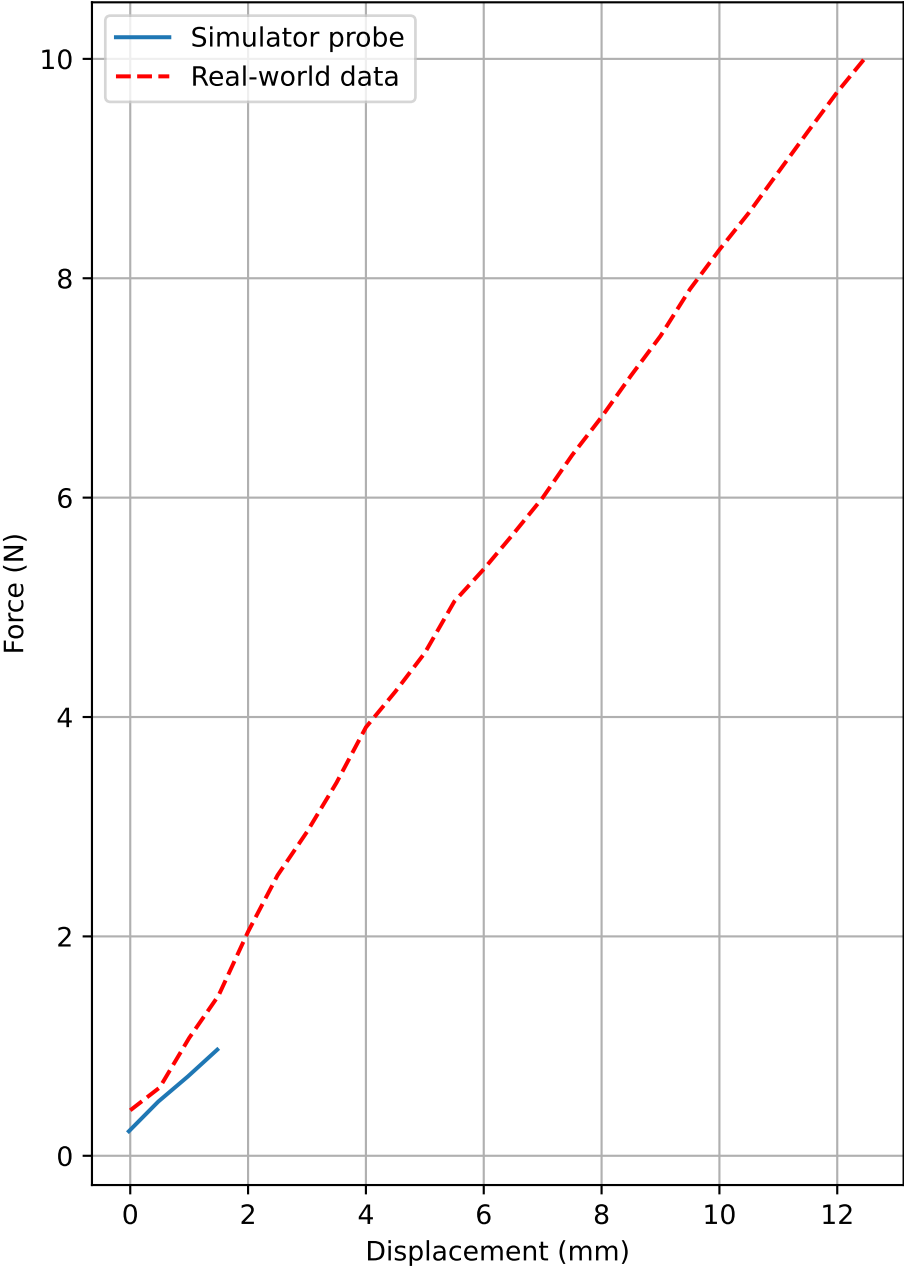
Actuator Force vs. Displacement
