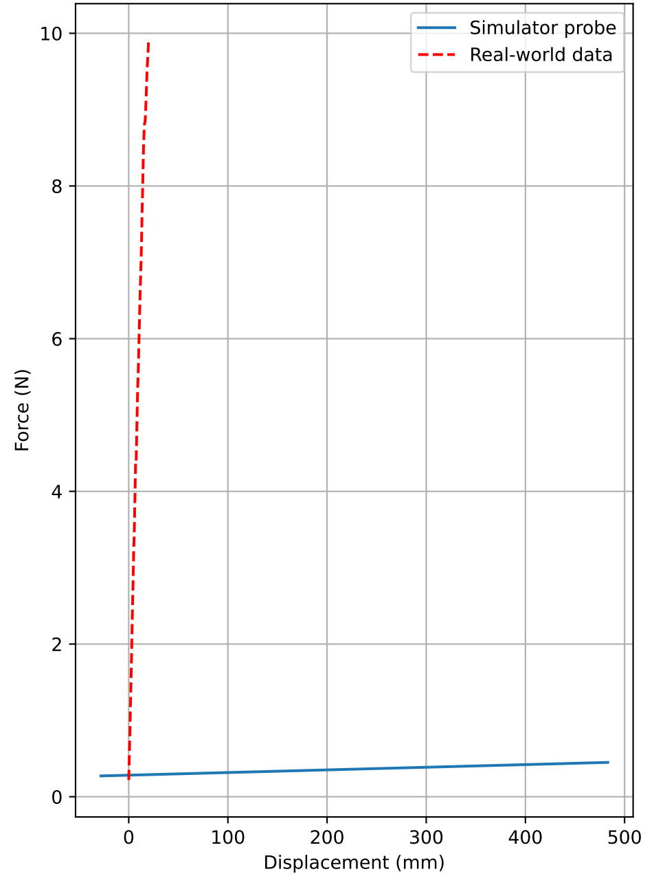
Actuator Force vs. Displacement
