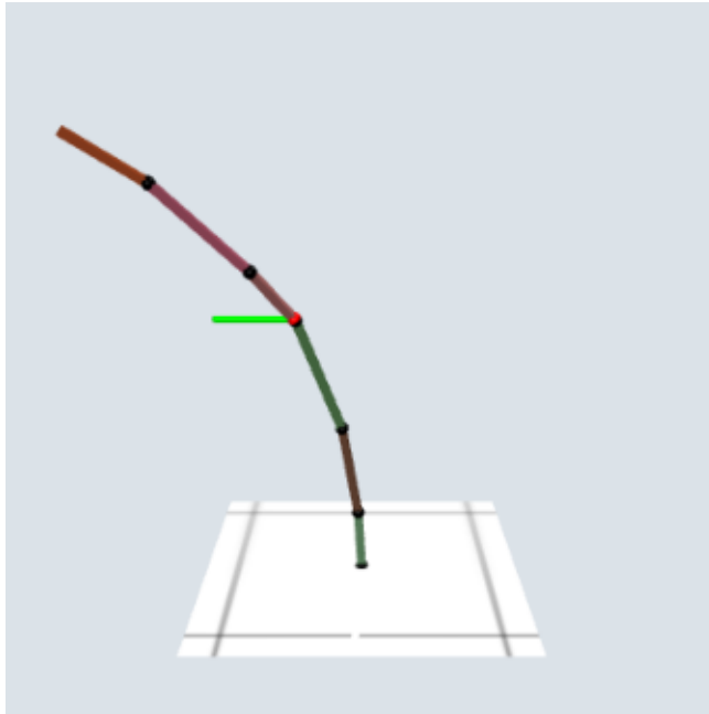
MuJoCo Model
