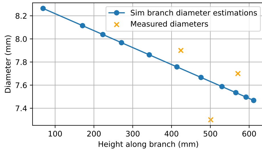
Branch Diameter Estimation, R^2 = 0.12
