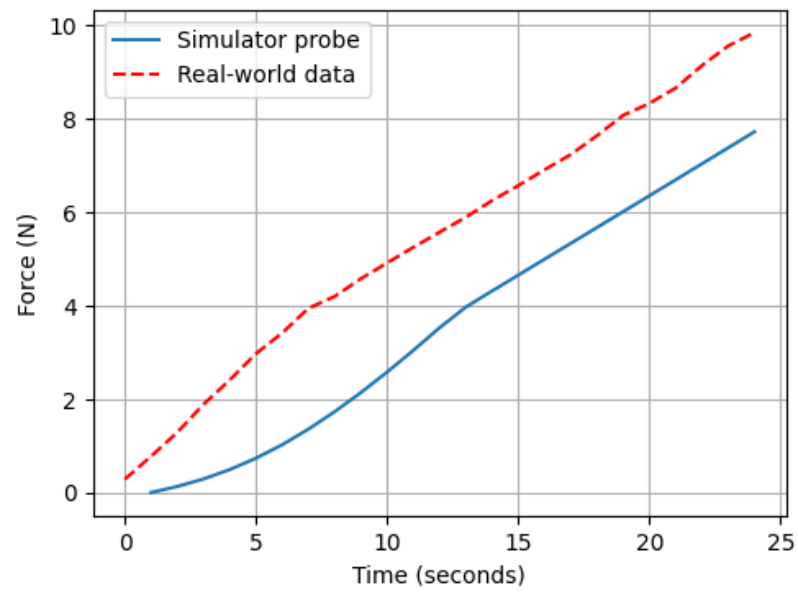
Actuator Force vs. Time
