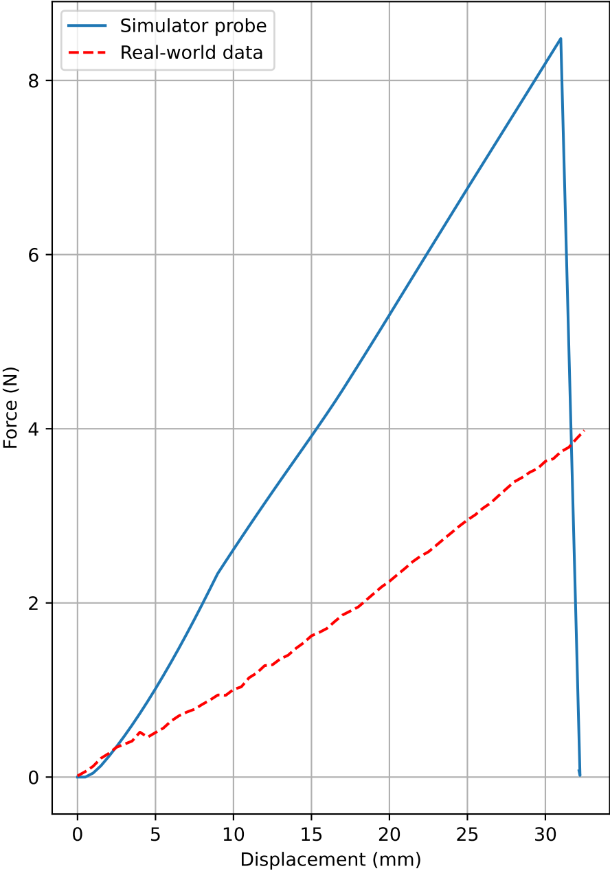
Actuator Force vs. Displacement
