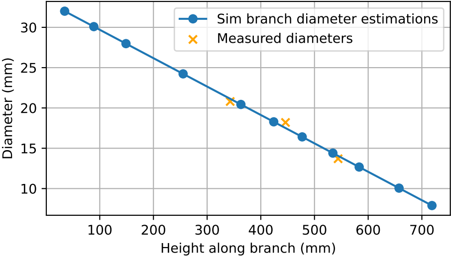
Branch Diameter Estimation, R^2 = 0.97
