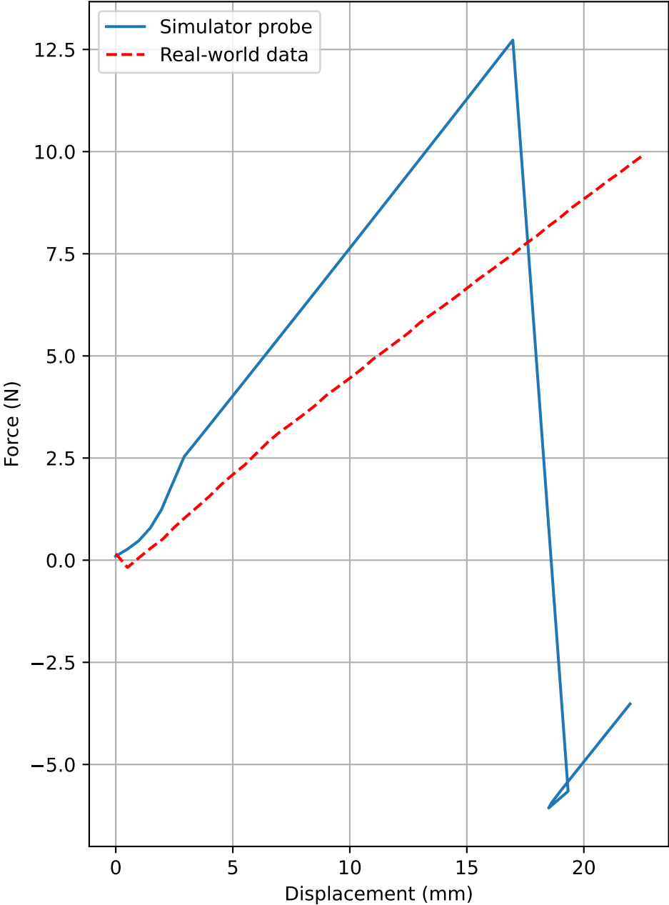
Actuator Force vs. Displacement
