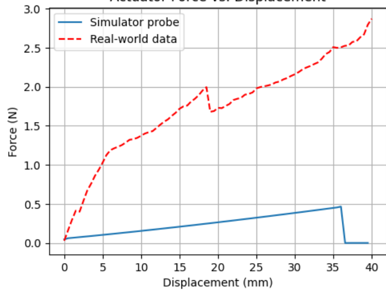
Actuator Force vs. Displacement
