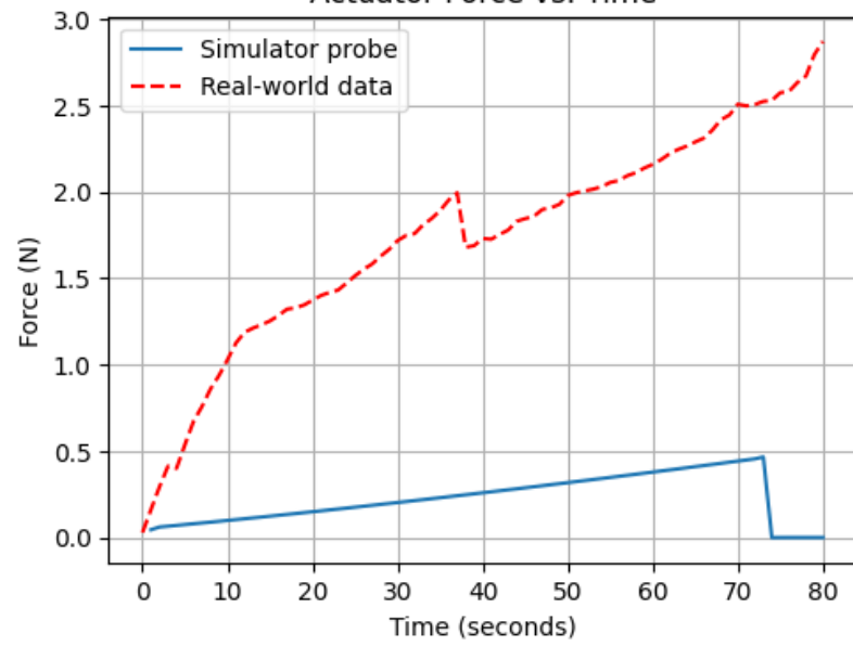
Actuator Force vs. Time
