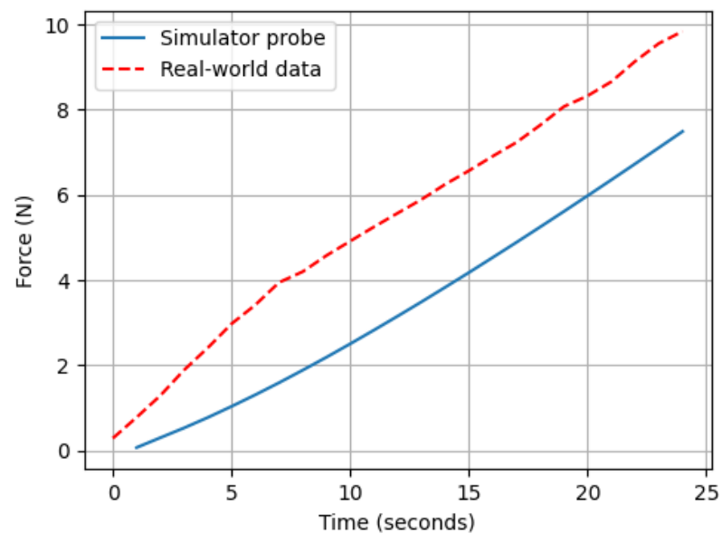
Actuator Force vs. Time
