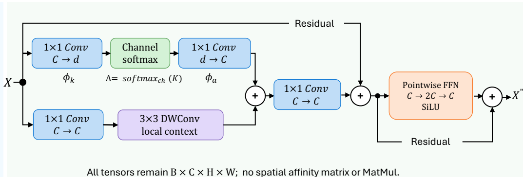
(b) DLABlock: channel mixing + local context
