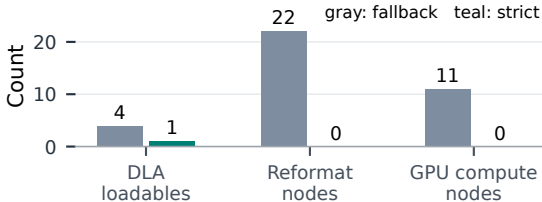
(b) Optimized engine inspection
