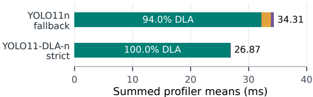
(a) Separately profiled engine
