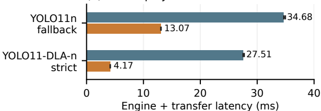
(b) DLA deployment
