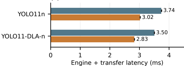
(b) DLA deployment
