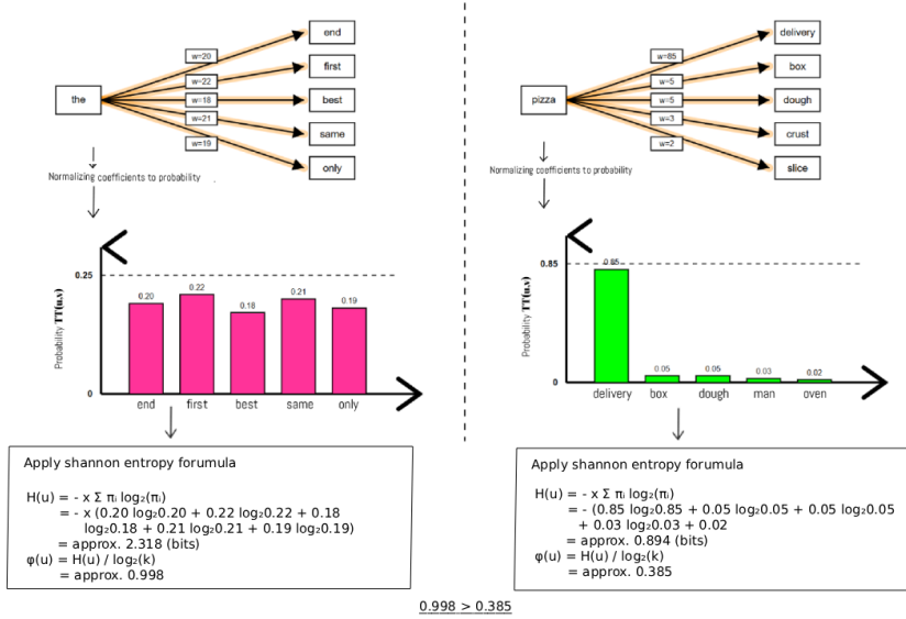
Figure 6. Illustrative comparison of high- and low-dispersion node connectivity and the corresponding Shannon-entropy values used in the seed construction process.
