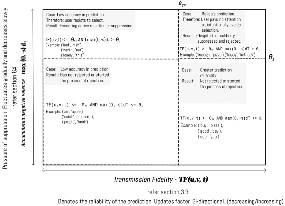
Figure 1. Illustration of transmission fidelity as a measure of prediction reliability, including the distinction between low- and high-reliability edge behavior.
