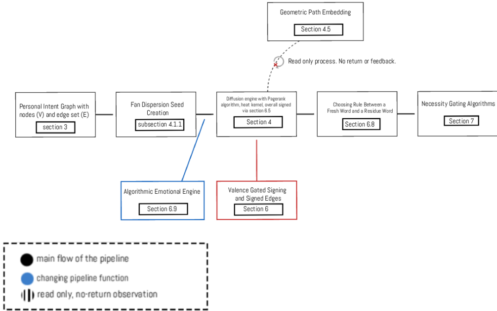
Figure 5. Overview of the IntentSpider processing architecture, showing the relationship between personalization, diffusion, valence, necessity gating, and the proposed downstream processes.
