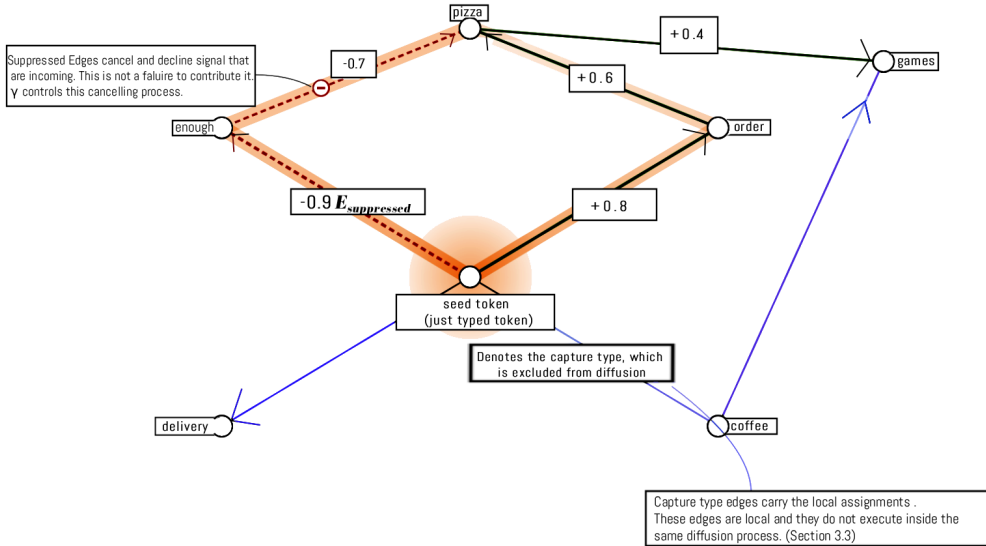
Figure 2. Illustration of transmission-type and capture-type edge roles, including the diffusion path and the direct non-forwarding association.
