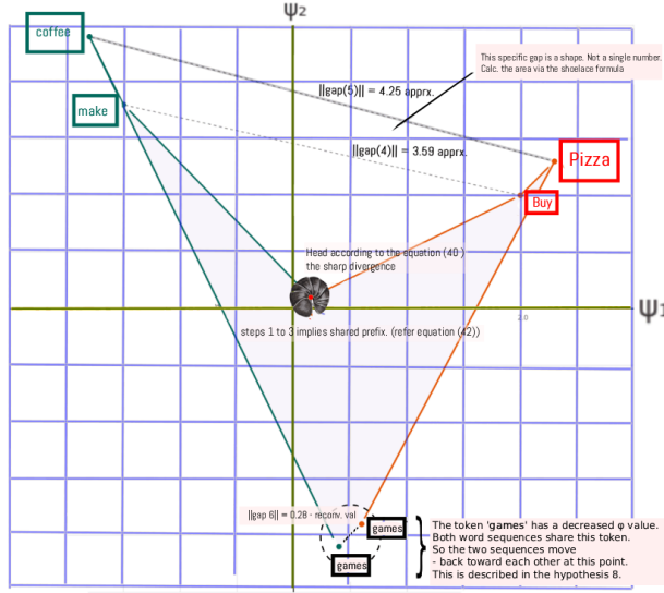
Figure 8. Illustrative two-dimensional trajectories produced by sequences of next-word distributions in the embedded intent graph.
