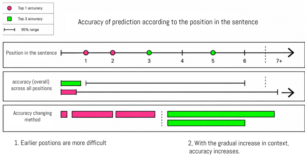
Figure 19. Prediction accuracy according to the position of the next word in the sentence.
