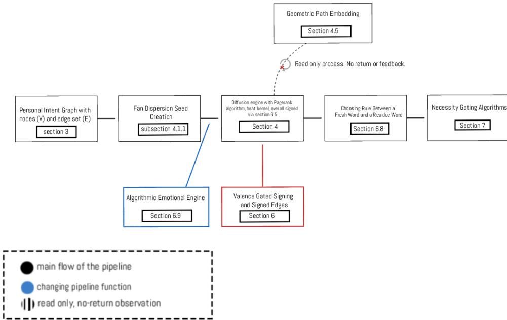
Figure 1. An Overview of the IntentSpider processing architecture
