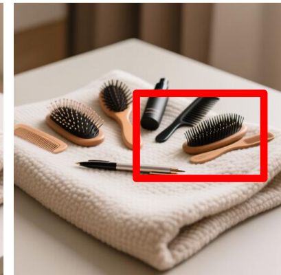
Qwen-Image
