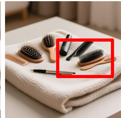
Qwen-Image
