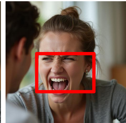
FLUX.1
