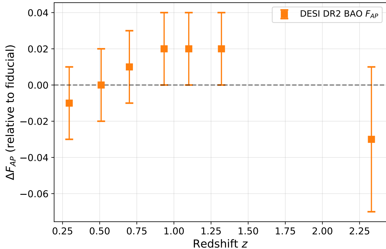
BAO AP Residuals: F_{AP}
