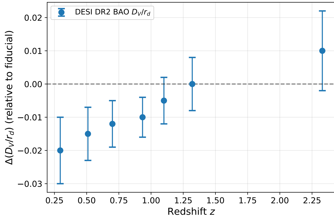
BAO Distance Residuals: D_V/r_d
