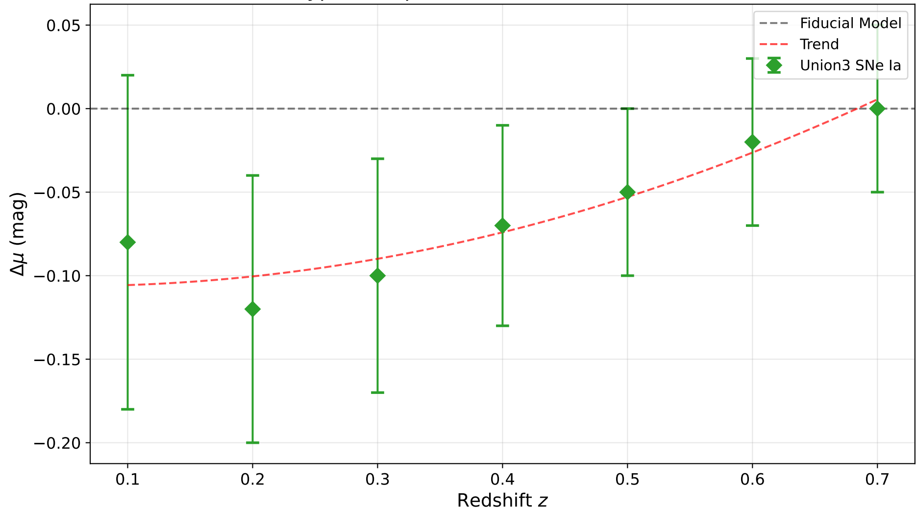
Union3 Type Ia Supernova Distance Modulus Residuals
