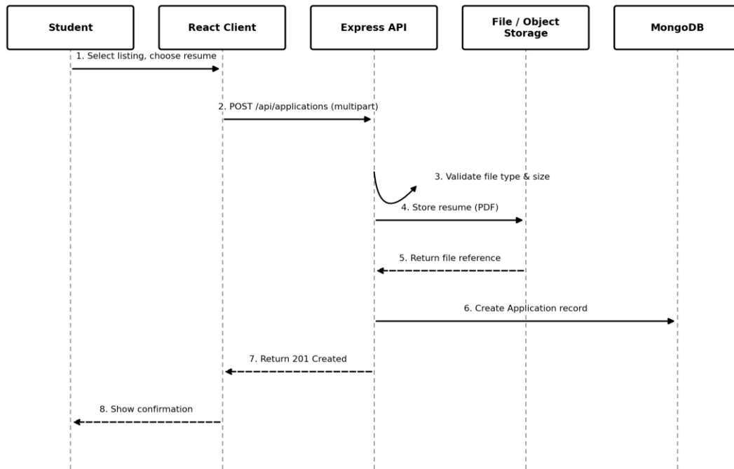
Sequence Diagram 2 — Apply to Internship (Resume Upload)
