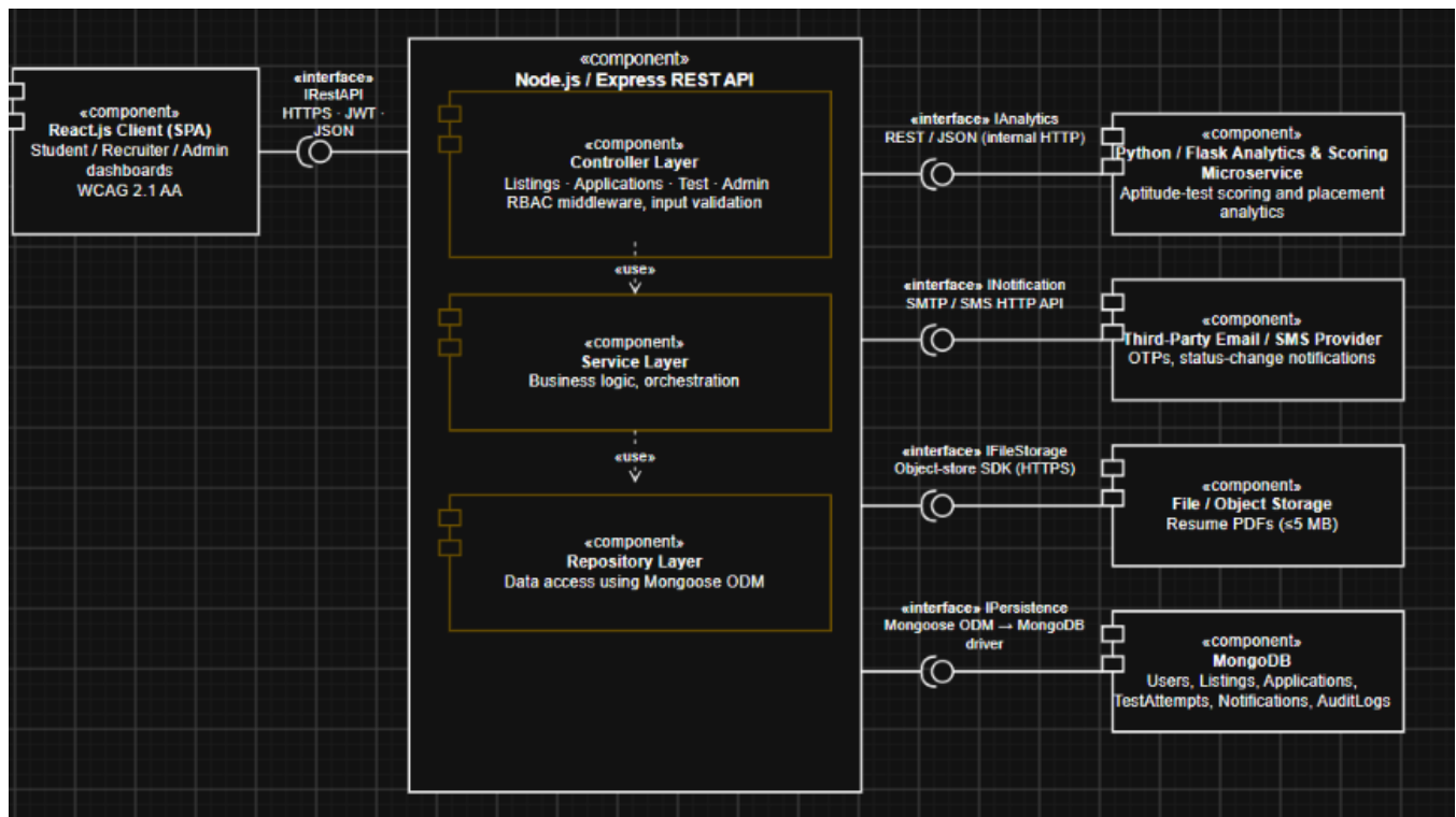
Figure 1: IPP Component Diagram
