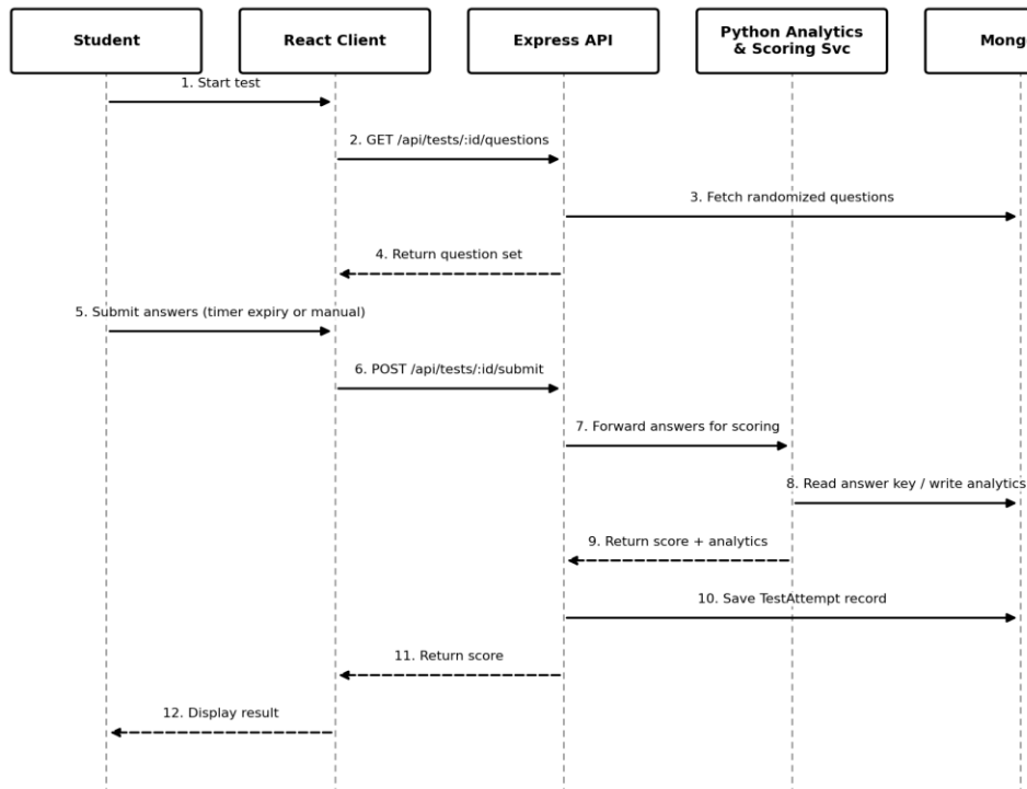
Sequence Diagram 3 — Take Aptitude Test & View Score
