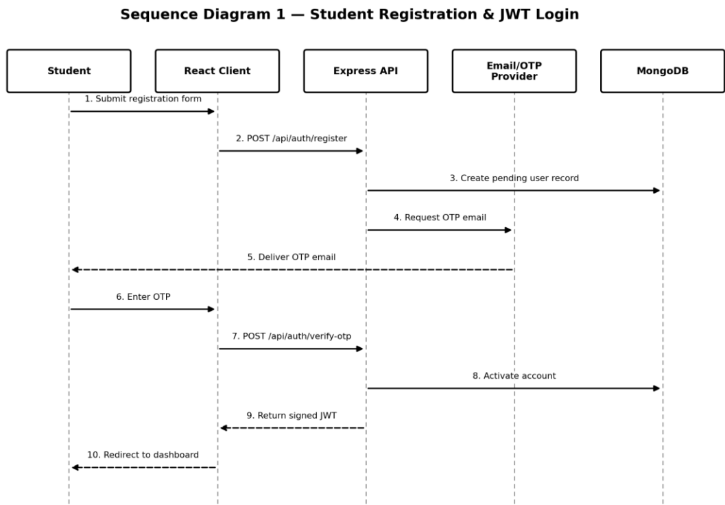
Figure 2: Sequence Diagram 1 — Student Registration & JWT Login
