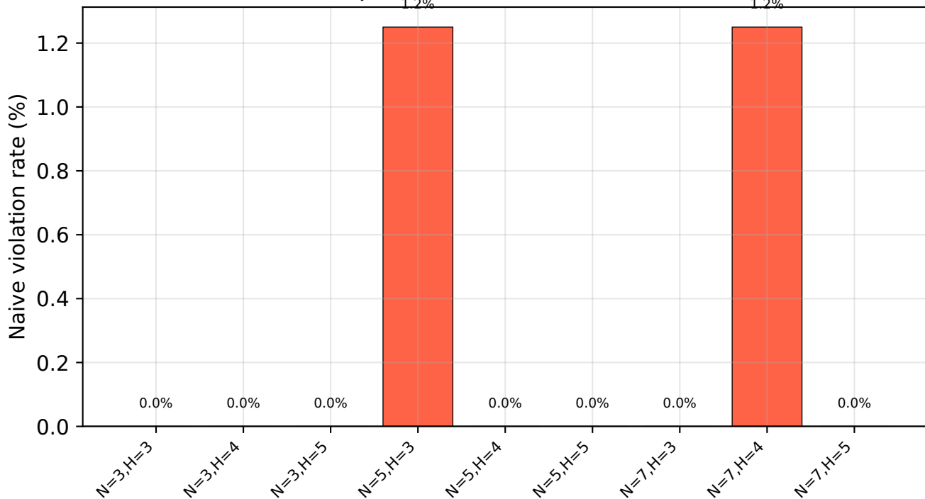
exp_06 Naive bound underbound rate per (N, H) setting (nonzero = prefix drift causes missed \tilde{W} mass)
