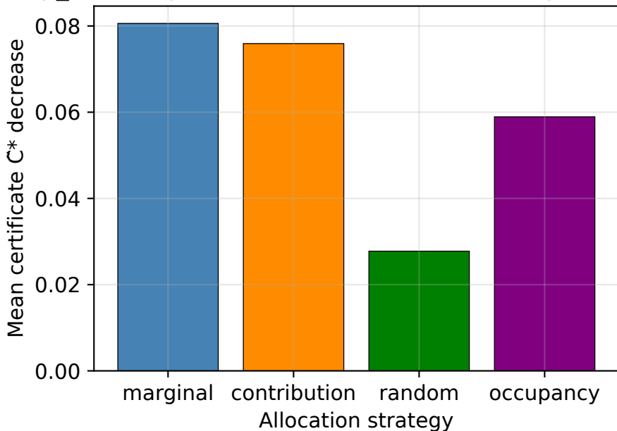
exp_09 Group1: Mean certificate decrease per strategy
