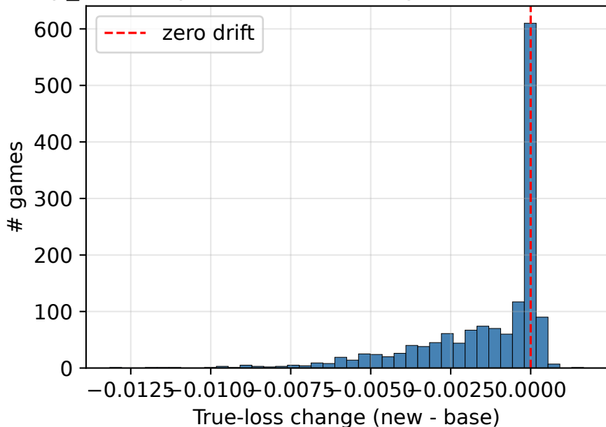
exp_09 Group3: True-loss change (drift events=374)
