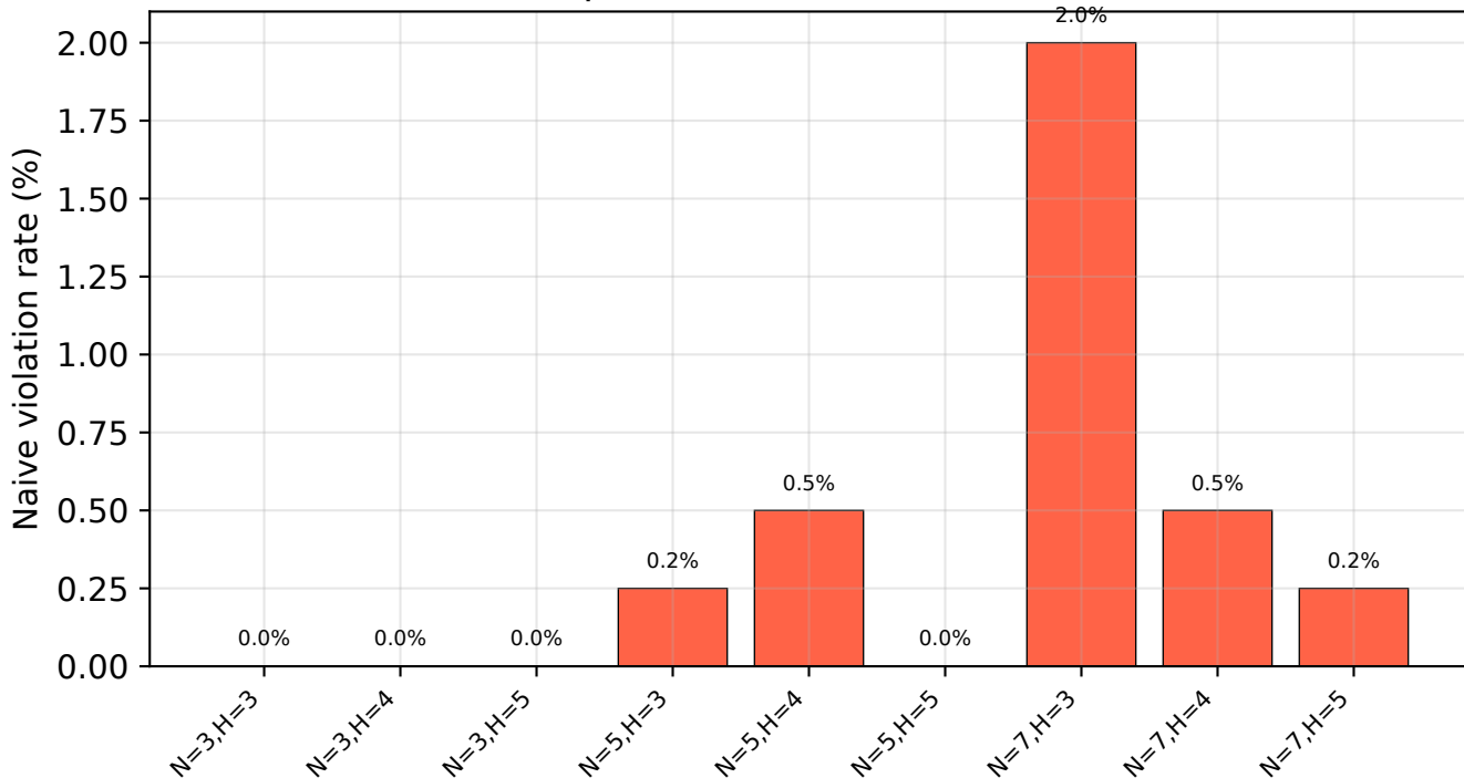
exp_06 Naive bound underbound rate per (N, H) setting (nonzero = prefix drift causes missed \tilde{W} mass)
