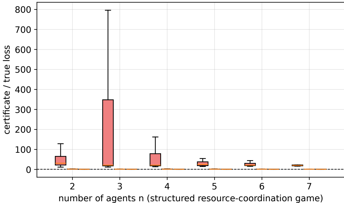
Structured game: chain tightness vs. agent count n (red=C0/L, yellow=C1/L, green=C2/L)
