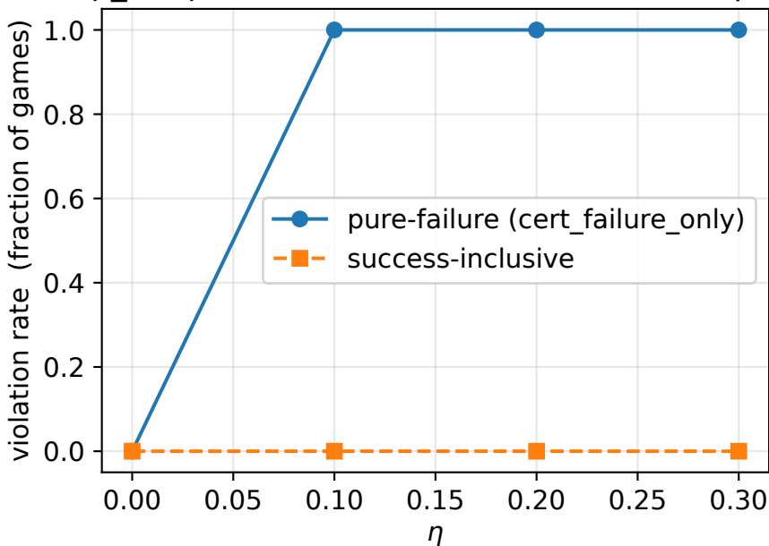
exp_02 pure-failure vs success-inclusive ( \eta > 0 )
