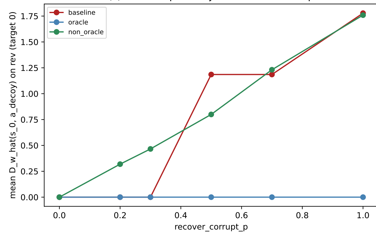
(c) Decision-point asymmetric error vs rcp
