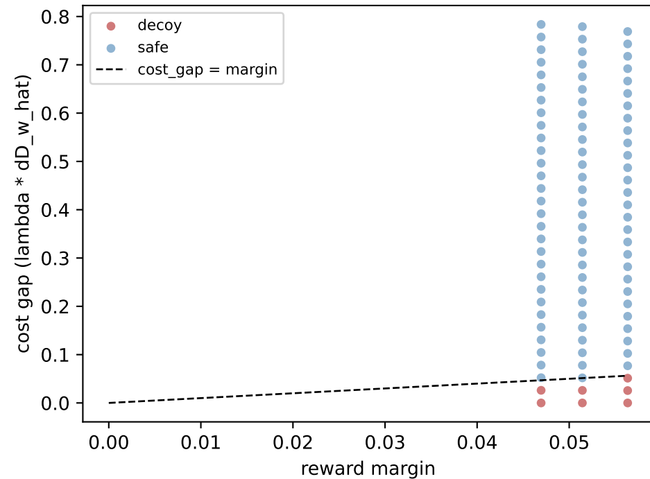
(c) margin theorem (0 violations)
