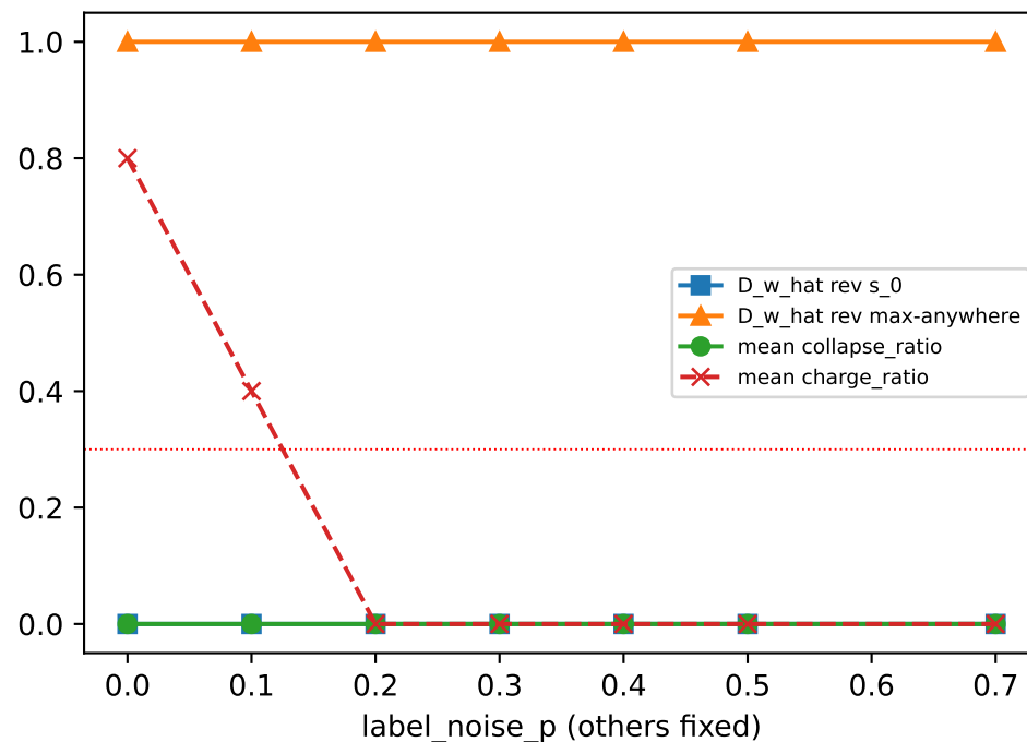
(e) Ablation -- label noise
