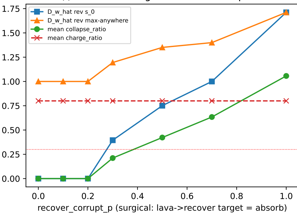
(i) Ablation -- surgical recover corruption
