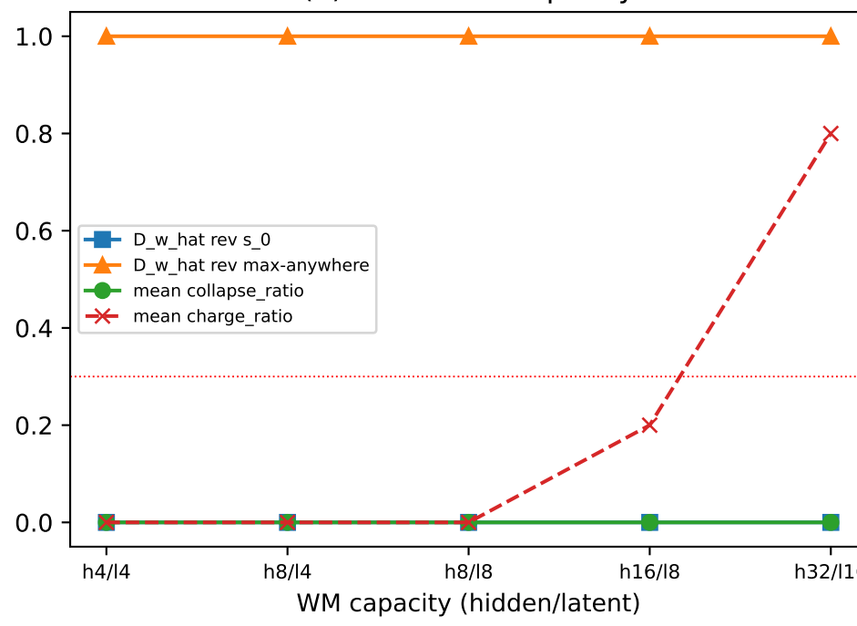
(h) Ablation -- capacity
