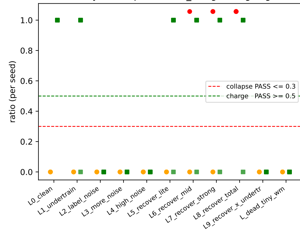
(g) Ablation -- training budget
