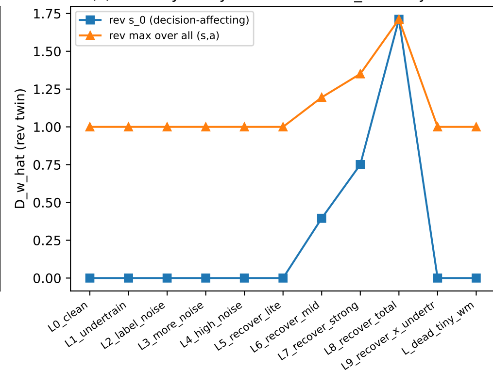
(f) Ablation -- obs noise
