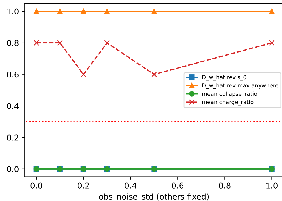
(f) Ablation -- obs noise
