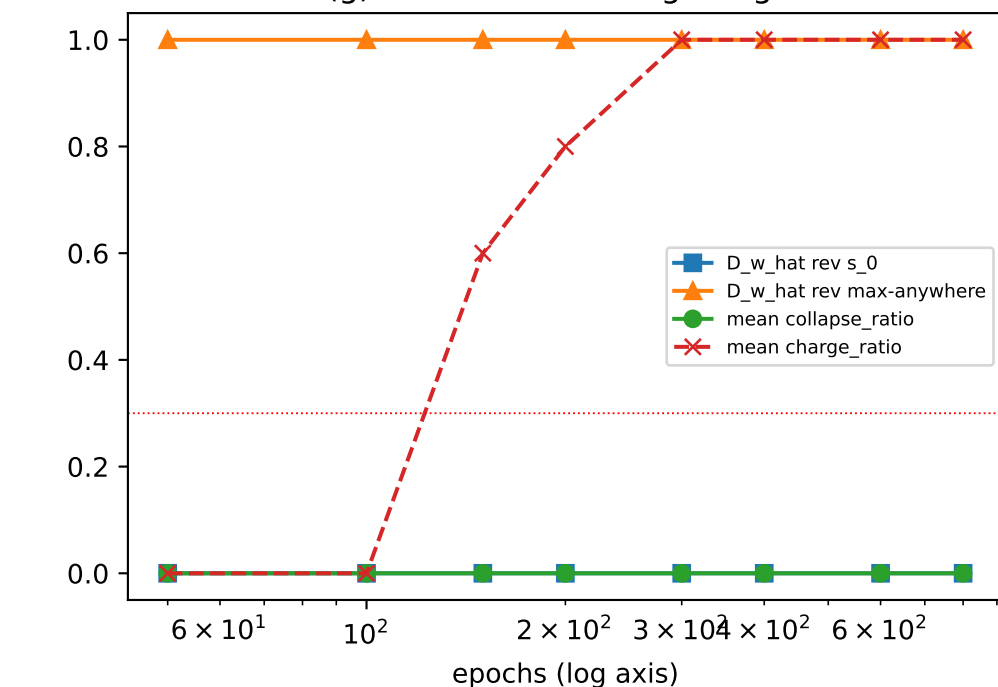
(g) Ablation -- training budget
