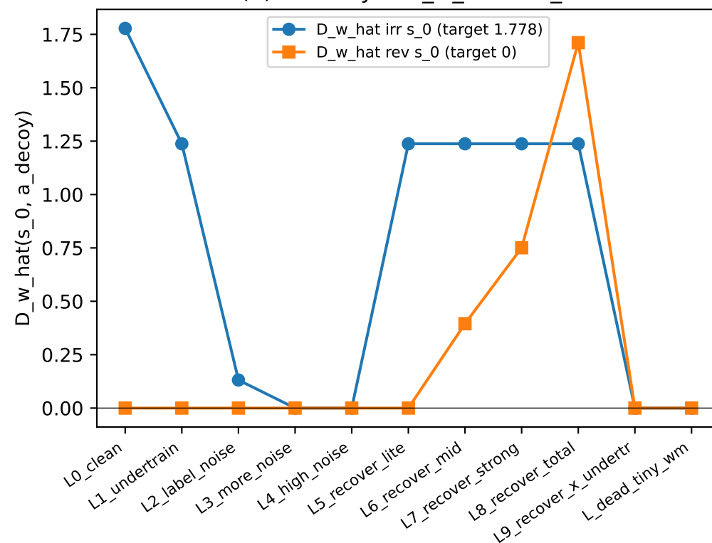
(e) Ablation -- label noise
