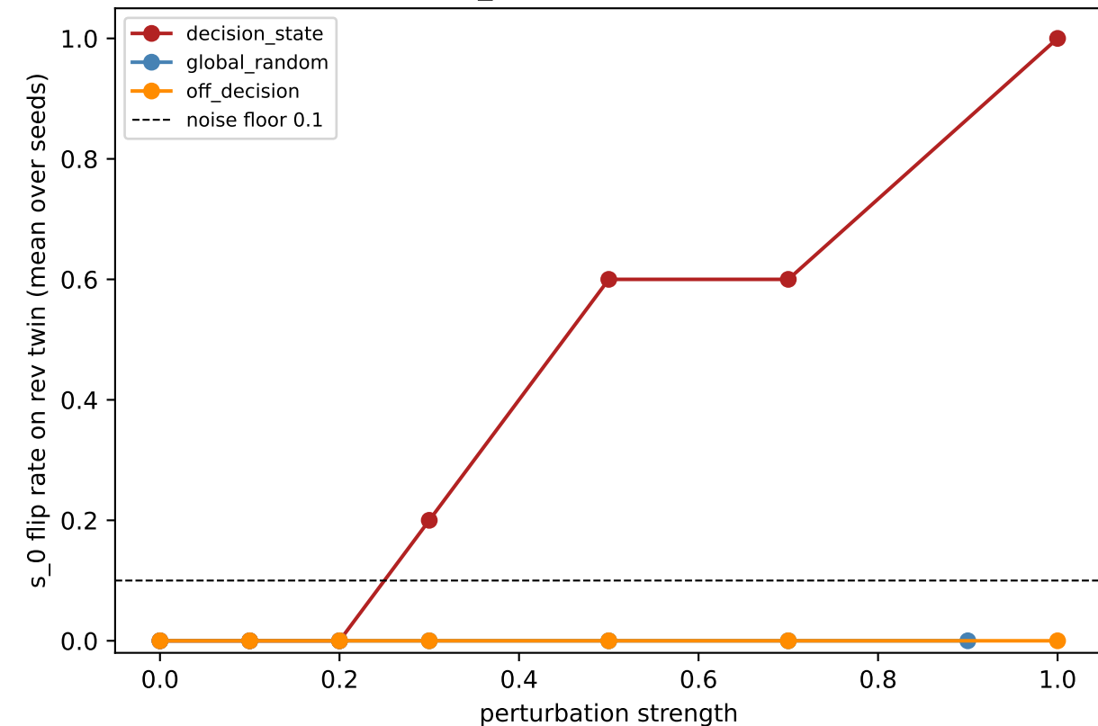
(a) s_0 flip rate vs strength
