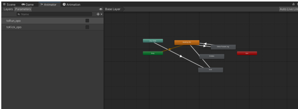
Fig. 3.1 – My project: Animator state machine of the opponent (Entry → breaking idle; Strike Forward Jog, Dribble, kick) with parameters toRun_opo and toKick_opo .
