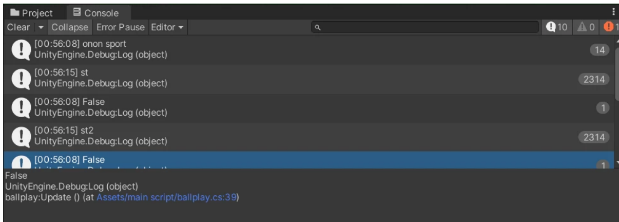
Fig. 8.1 – Console from my project during play: the per-frame debug lines from ballplay.Update() ("st", "st2") have each been logged 2314 times, plus Debug.Log(False) output – an avoidable CPU/GC cost found in the Console.
