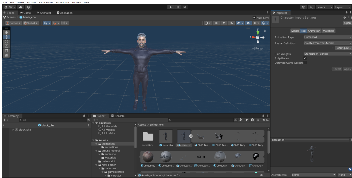
Fig. 2.2 – Model Importer, Rig tab of the character FBX (character.fbx): Animation Type = Humanoid , Avatar Definition = Create From This Model, so Unity builds an Avatar for retargeting animations.
