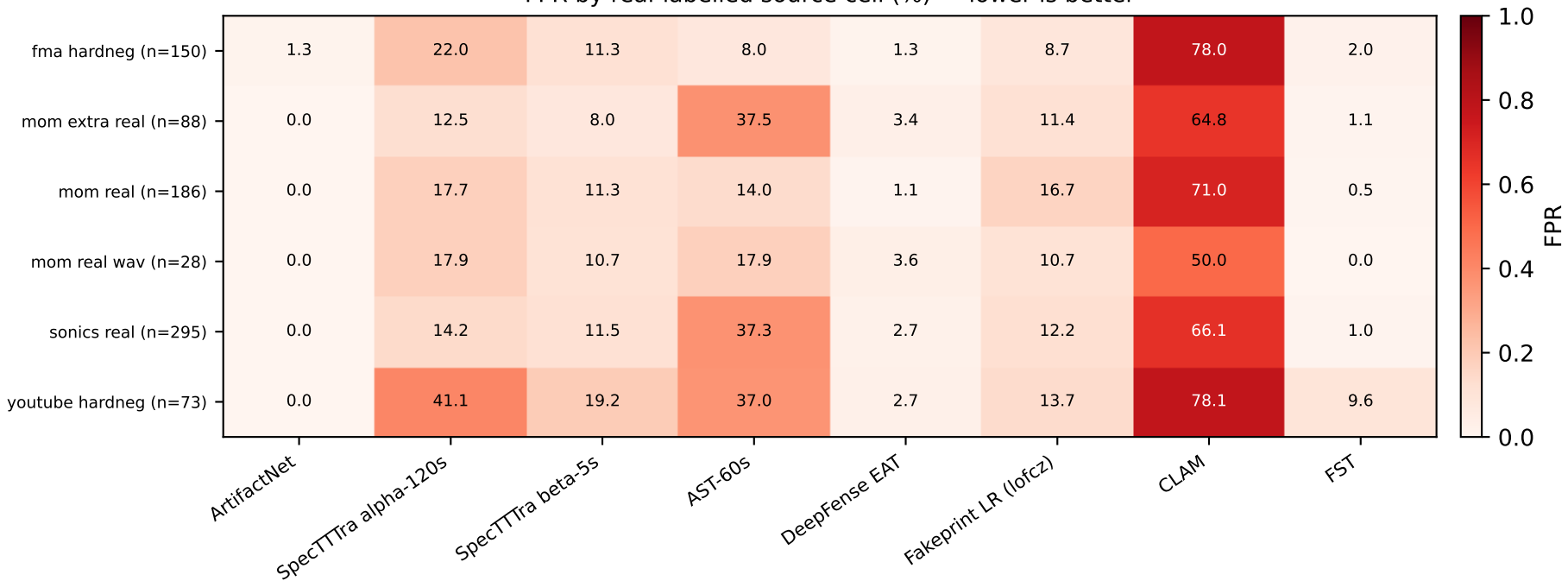
FPR by real-labelled source cell (%) — lower is better
