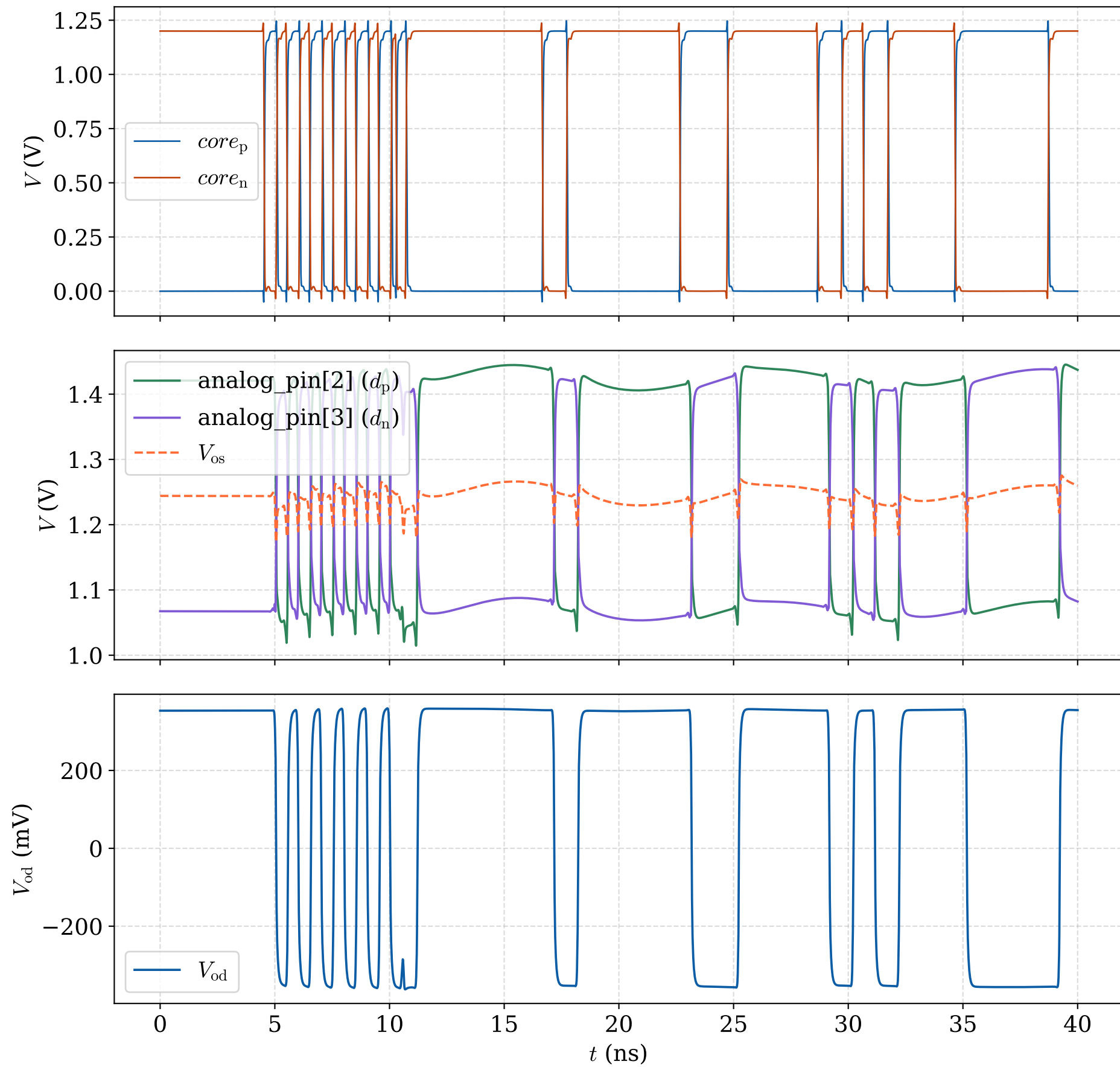
Chipalooza 2026 - pattern generator into the LVDS driver
