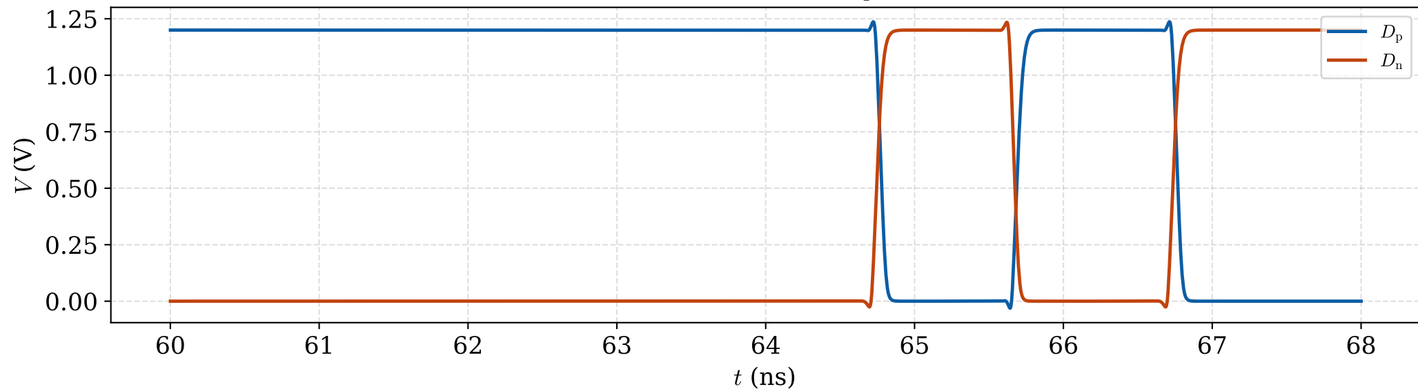
PRBS-7 at 1 Gb/s, into the 170 fF pre-driver load
