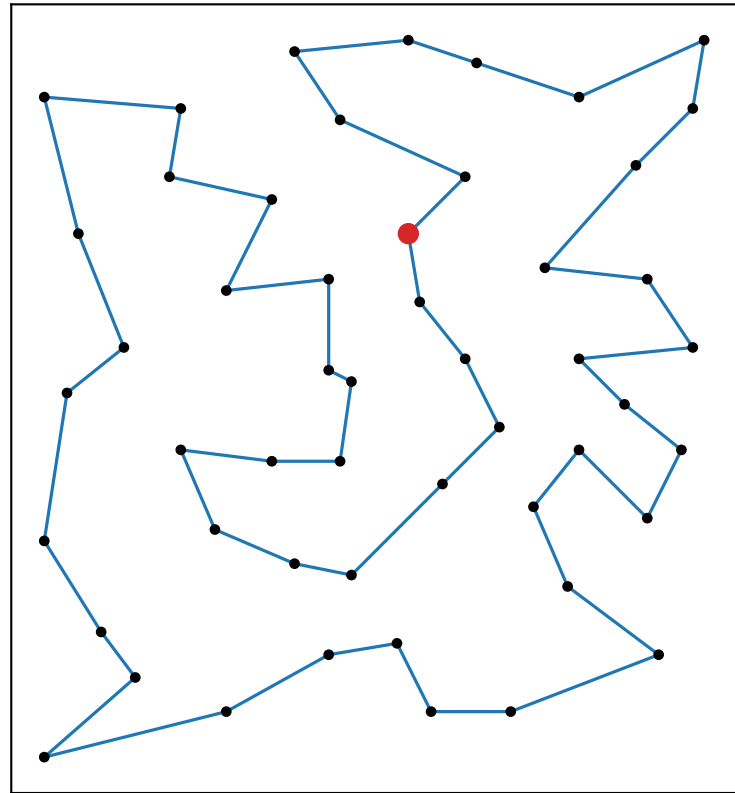
optimum: L = 426
