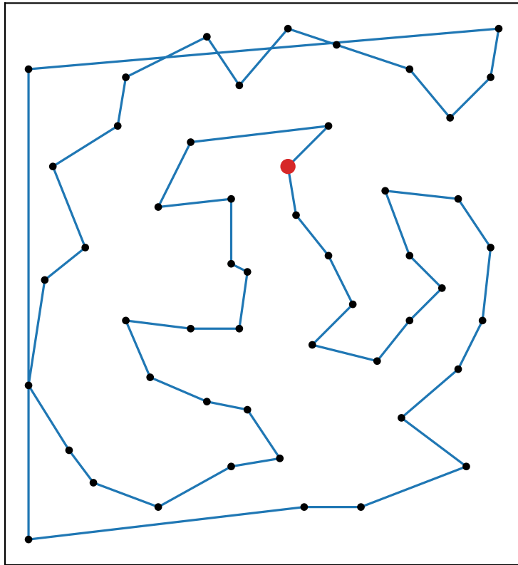
greedy edge: L = 531
