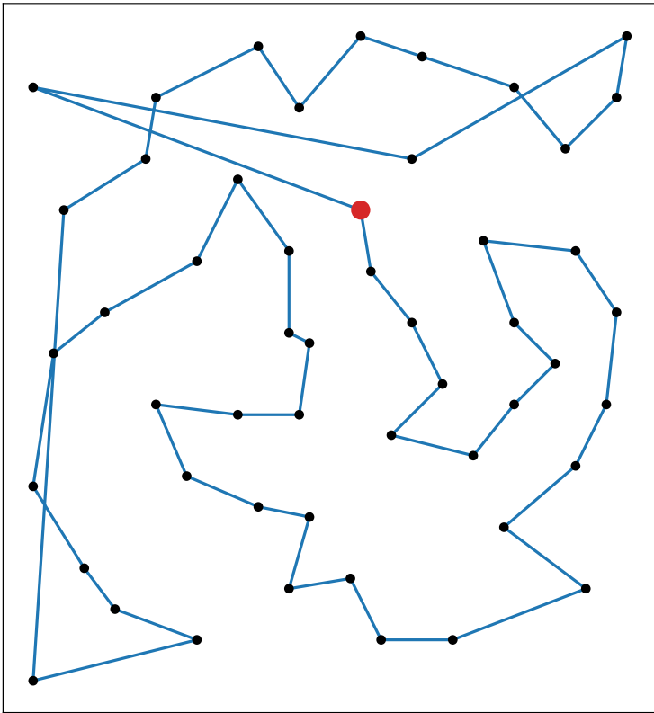
nearest neighbour: L = 511
