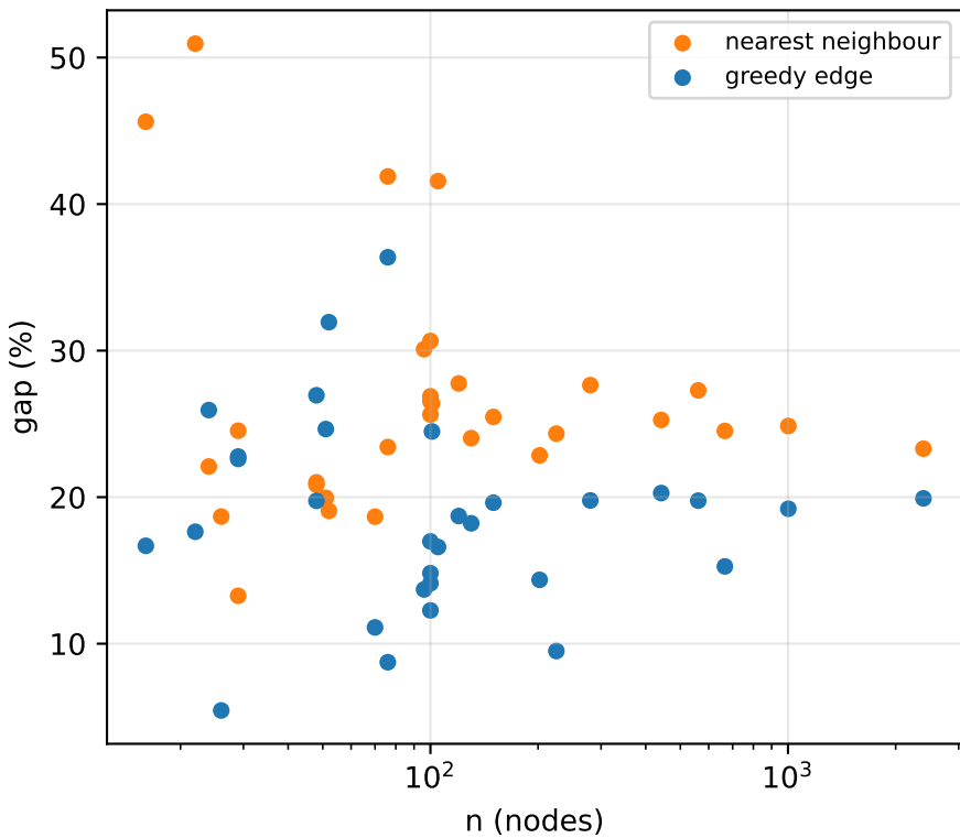
Gap to the optimum (31 instances, without brg180)
