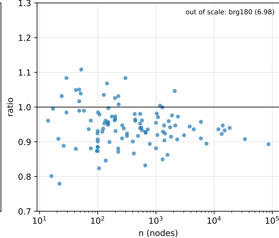
Greedy length / nearest-neighbour length
