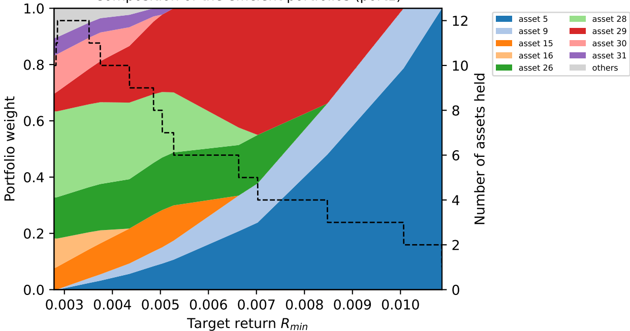
Composition of the efficient portfolios (port1)
