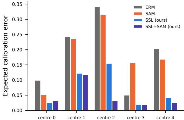
a Both SSL arms beat ERM and SAM at every hospital
