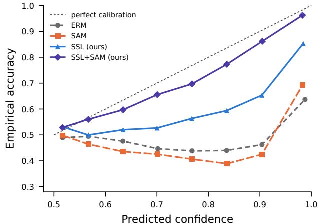
b Reliability at the hardest hospital (centre 2)
