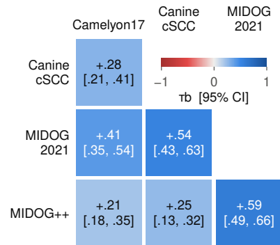
a Kendall \tau_b between cohort rankings
