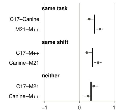
c \tau_b by cohort-pair type
