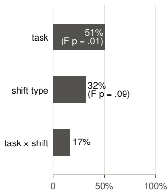
b Split of between-cohort SS
