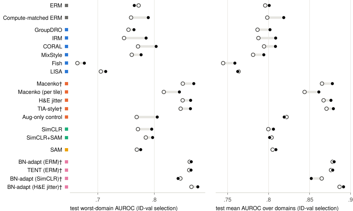
a worst-domain AUROC ( \tau_b = 0.78 )
