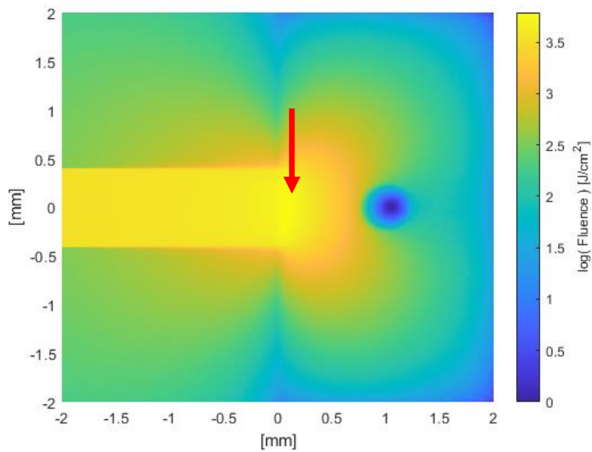
Peak value at the epidermis interface is approximately 3.8.
