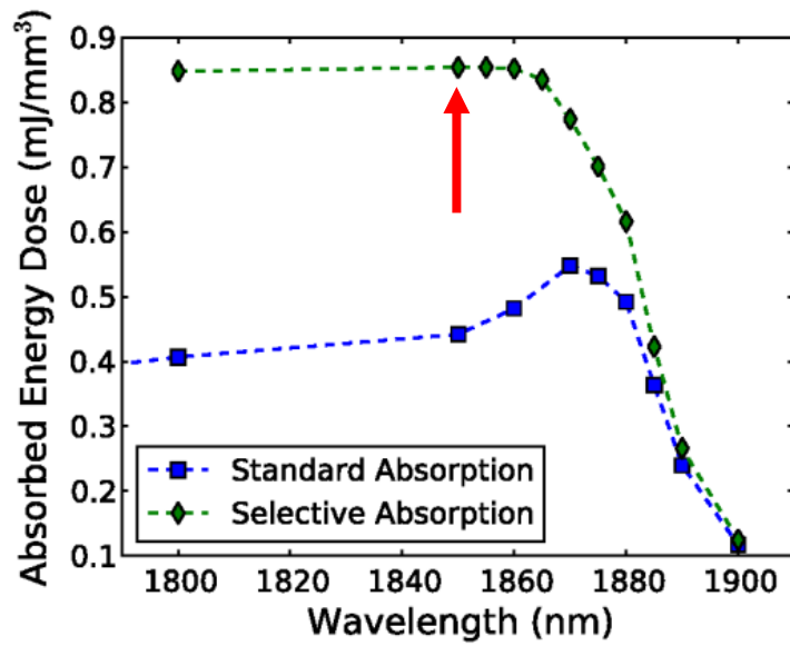
Figure 8 – Peak absorbed energy in the middle of the nerve layer at 1850 nm is approximately 0.85 mJ/mm 3
