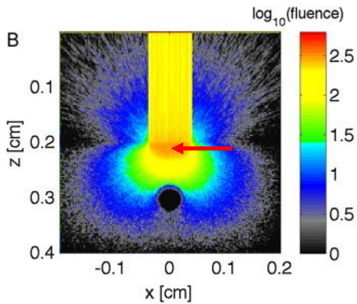
Figure 1 - Peak value at the epidermis-water interface is approximately 2.5.
