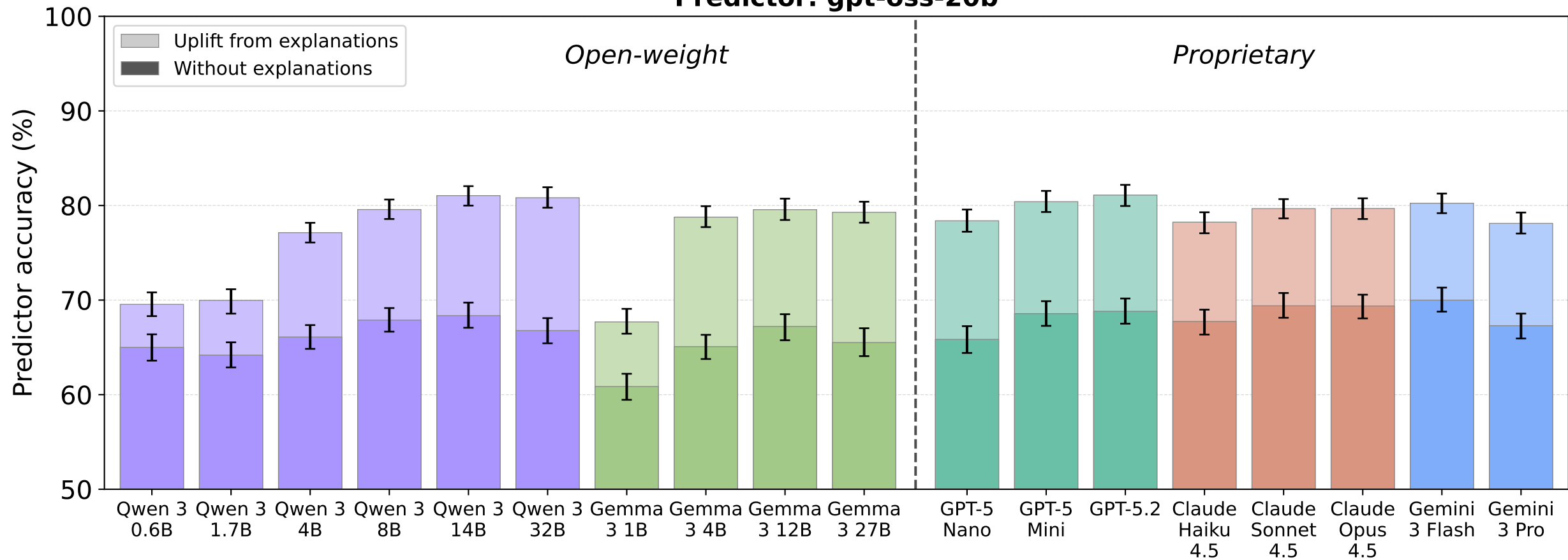
Predictor: gpt-oss-20b
