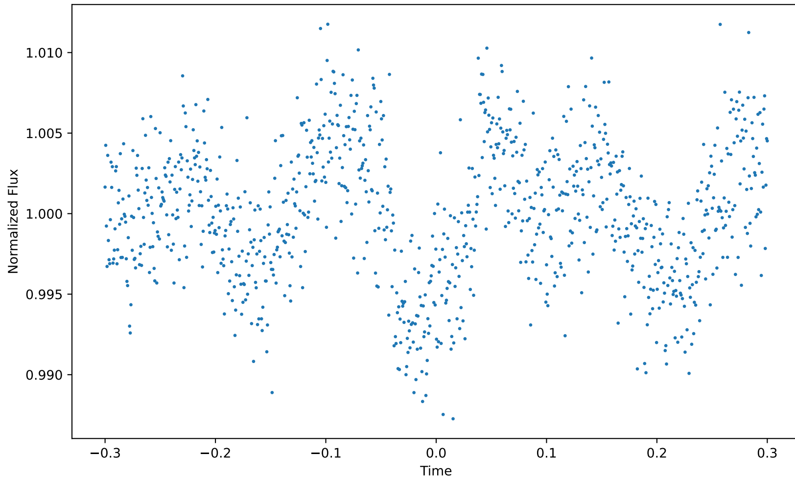
Artifact-Removed Light Curve
