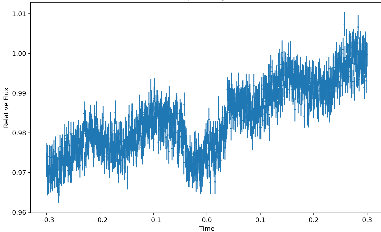
Raw Exoplanet Light Curve
