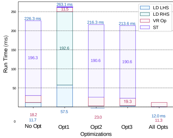
Figure 12: Binary matrix multiplication runtime breakdown with different optimizations. Opt1: communication-aware reduction mapping. Opt2: DMA Coalescing. Opt3: broadcast-friendly data layout.
