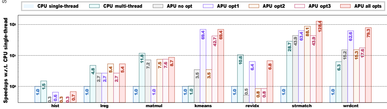
Figure 13: Latency comparison across workloads from the Phoenix Benchmark Suite, normalized to the single-threaded Intel Xeon Gold CPU baseline. Opt1: communication-aware reduction mapping. Opt2: DMA Coalescing. Opt3: broadcast-friendly data layout.
