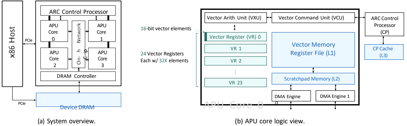
Figure 3: The GSI APU system and APU core logic view, the memory hierarchy is highlighted in blue. The APU consists of a control processor, four APU cores, and a four-level memory hierarchy. Each core has 24 vector registers (VR), and each VR has 32768 elements.
