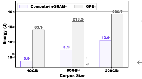
Figure 15: Top-5 retrieval process energy comparison with GPU. Results are measured on GSI Leda-E APU and NVIDIA A6000 GPU.
