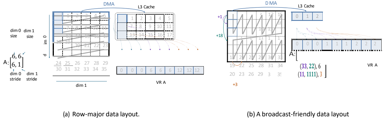
Figure 11: Broadcast-friendly data layout example – (a) a row-major data layout requires a lookup table of size 18. (b) A broadcast-friendly data layout only requires a lookup table size of size 3.
