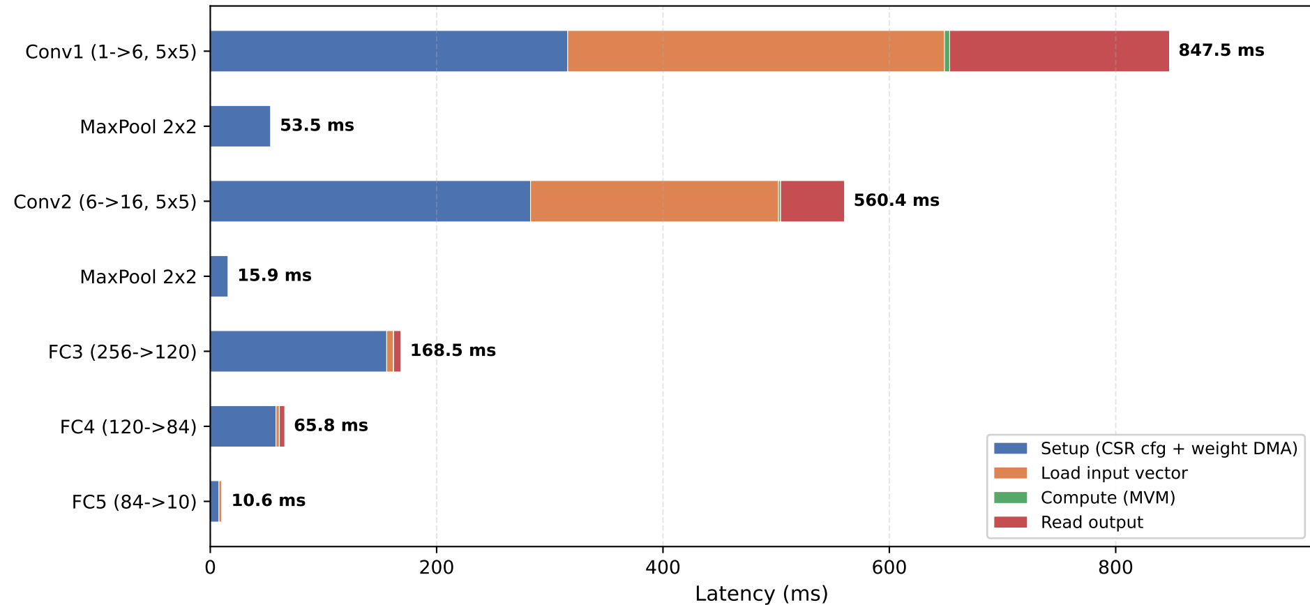
LeNet-5 Per-Layer Latency Breakdown (PYNQ-Z2, 60 MHz)
