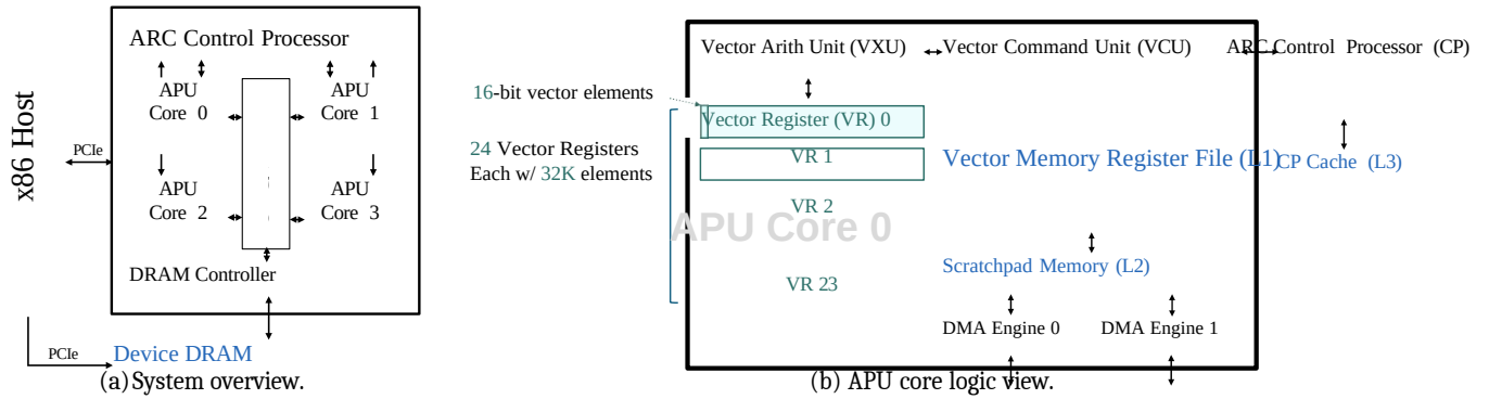
Figure 3: The GSI APU system and APU core logic view, the memory hierarchy is highlighted in blue. The APU consists of a control processor, four APU cores, and a four-level memory hierarchy. Each core has 24 vector registers (VR), and each VR has 32768 elements.
