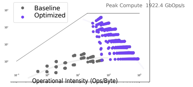
Figure 2: Performance of various matrix multiplication kernels on GSI APU, w/o data movement and data layout optimizations.
