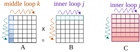
(a) Spatially unroll loop i .
