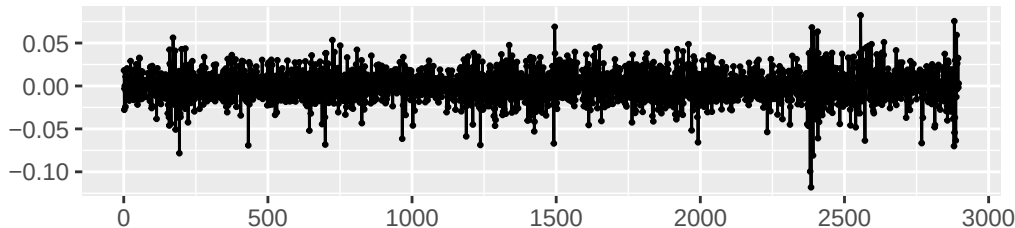
Residuals from ARIMA(0,0,0) with zero mean
